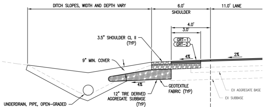
Typical Section
